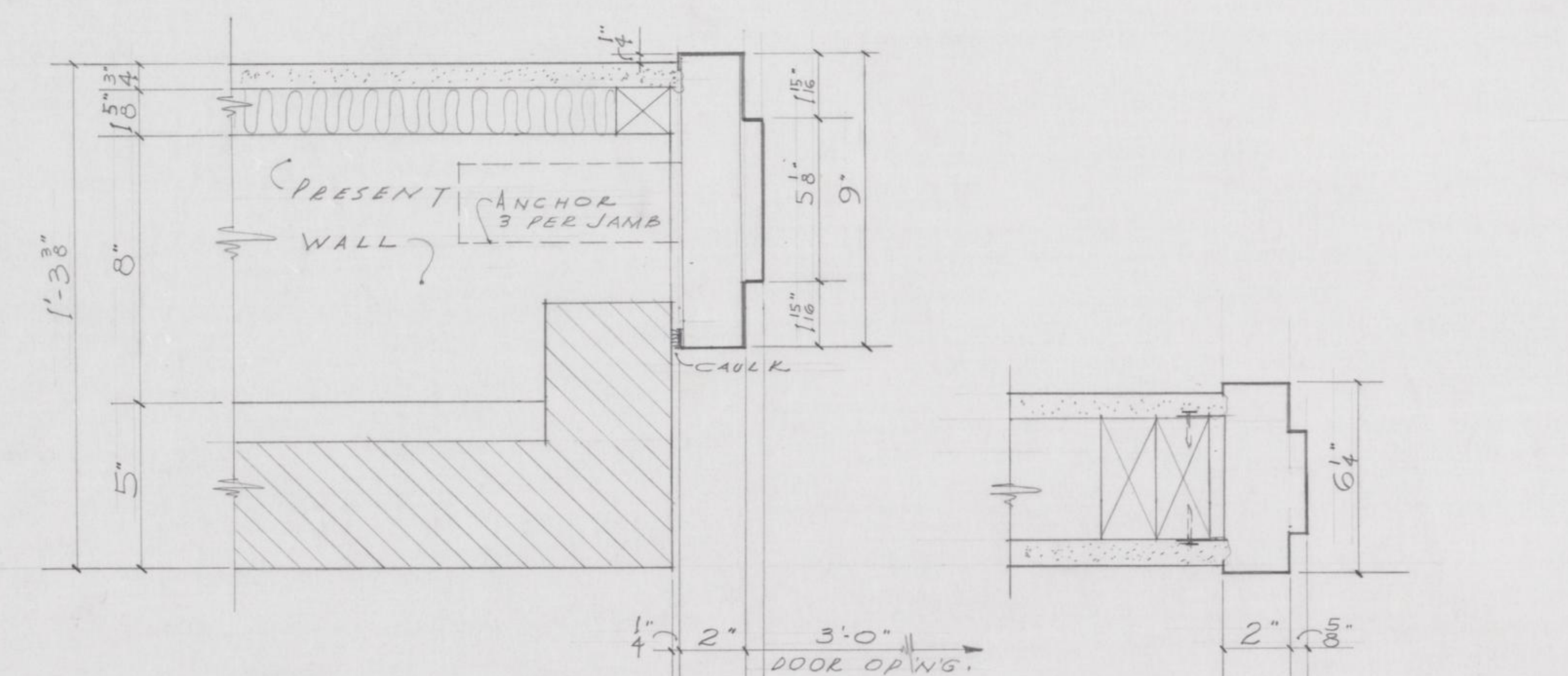
DETAIL OF FRAME FOR DOOR (2) TYPICAL INT. FRAME DET. FRAME FOR DOOR (3) SIMILAR DOOR FRAME DETAILS SC. 3" = 1'-0"
