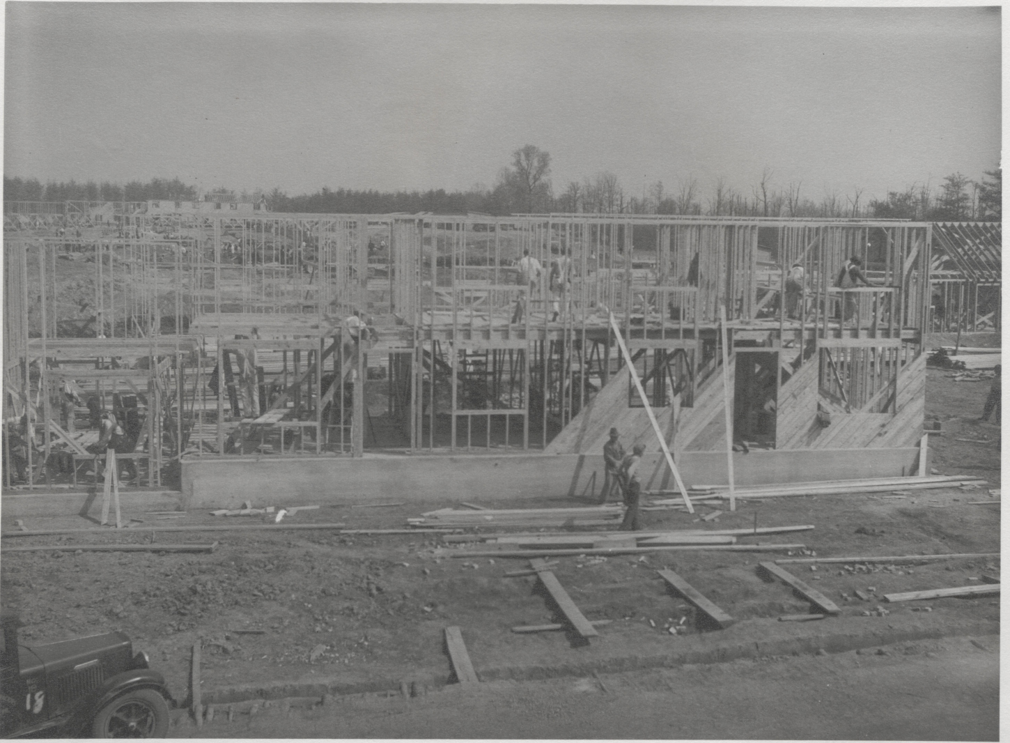
22. CINDER BLOCK 2nd FLOOR SLAB FORMING
