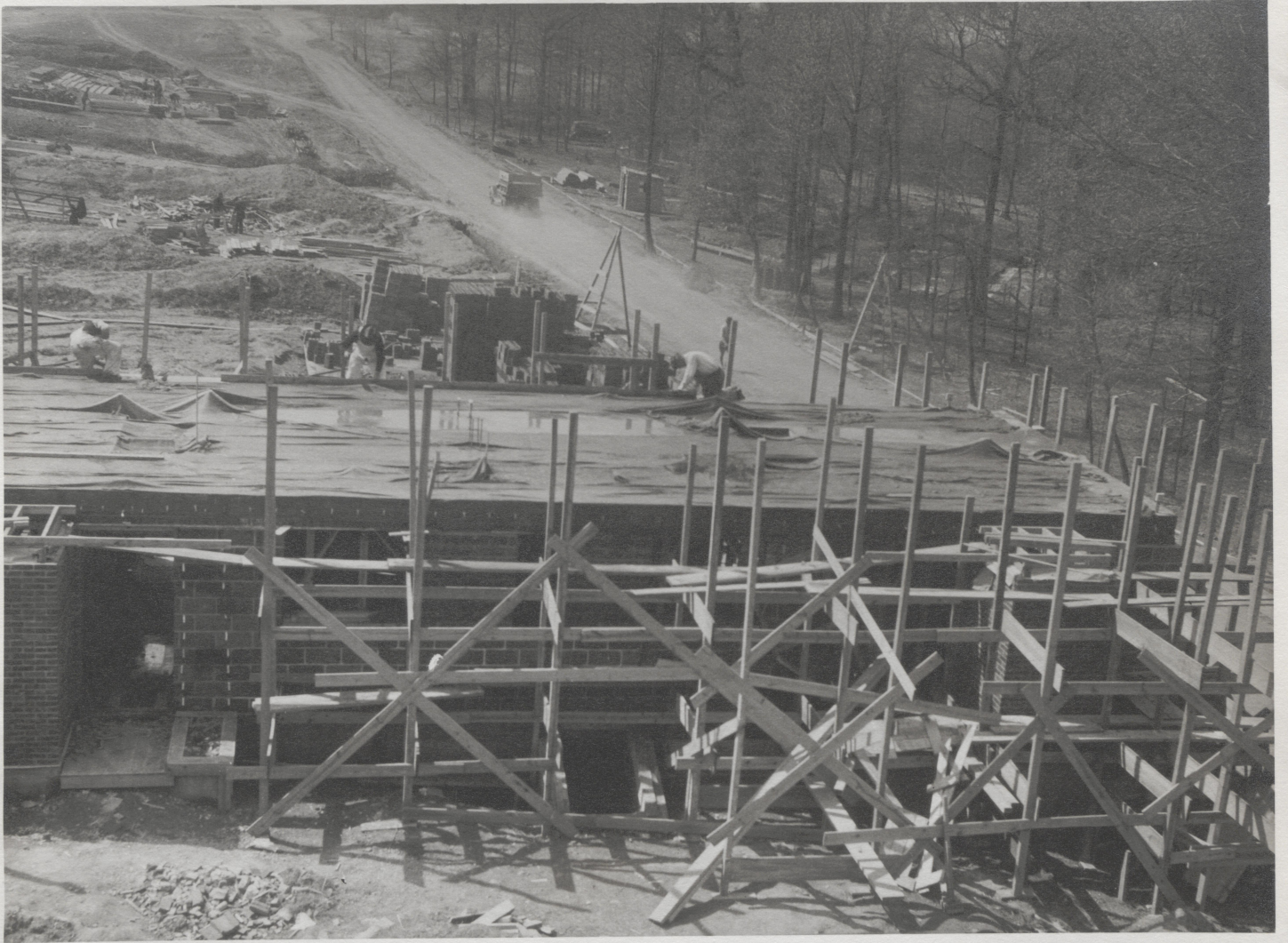
23. CINDER BLOCK 2nd FLOOR SLAB POURED
