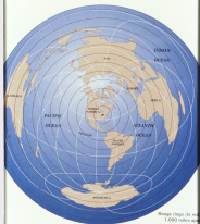
Azimuthal Equal-Area Projection Centered on Frankfort, Kentucky 38°12'N, 84°51'W
