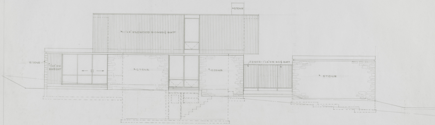
REAR ELEVATION
