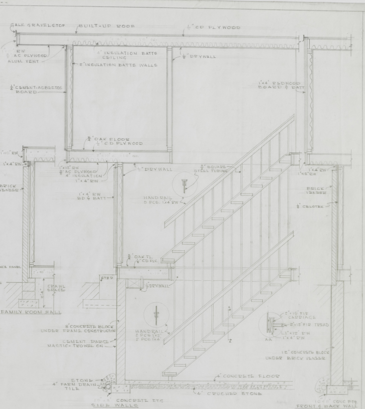
WALL SECTIONS SCALE 3/4" = 1'-0"
