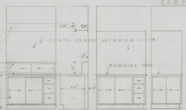
LEFT SIDE ELEVATION
