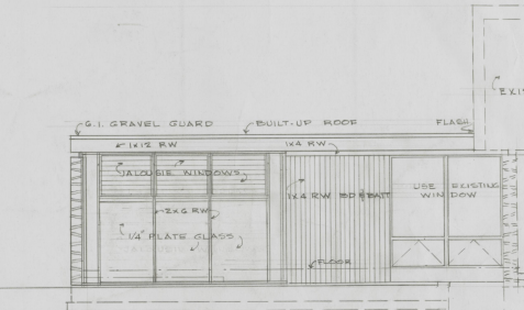
SIDE ELEVATION 1/4" = 1'-0"
