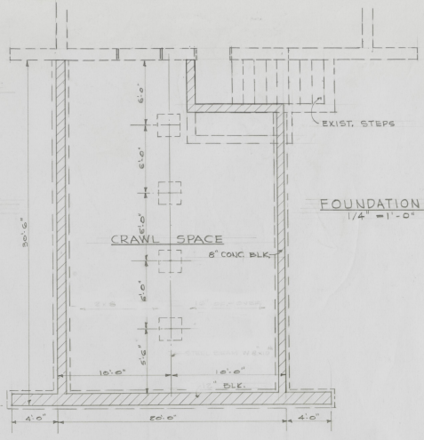
PLAN 1/4" = 1'-0"
