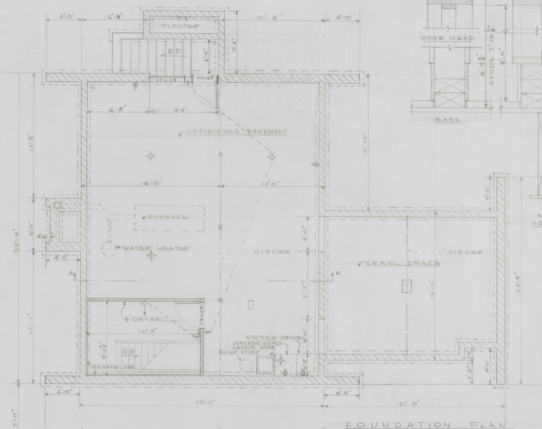
FOUNDATION PLAN
