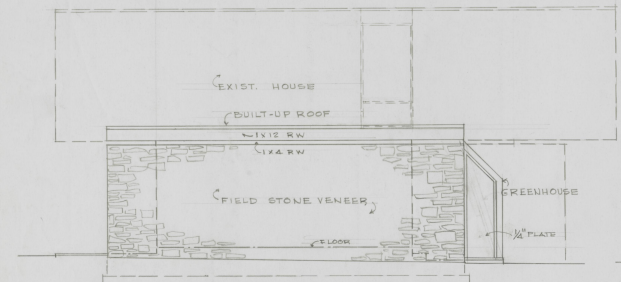
END ELEVATION 1/4" = 1'-0"
