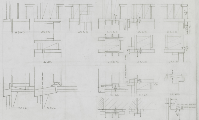
TRIM DETAILS SCALE 1/2" = 1'-0"
