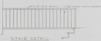
STAIR DETAIL
