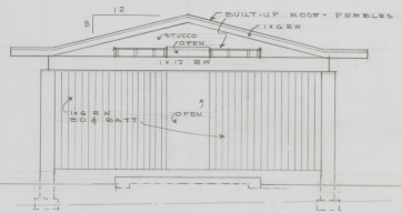
CARPORT LEFT SIDE ELEV.
