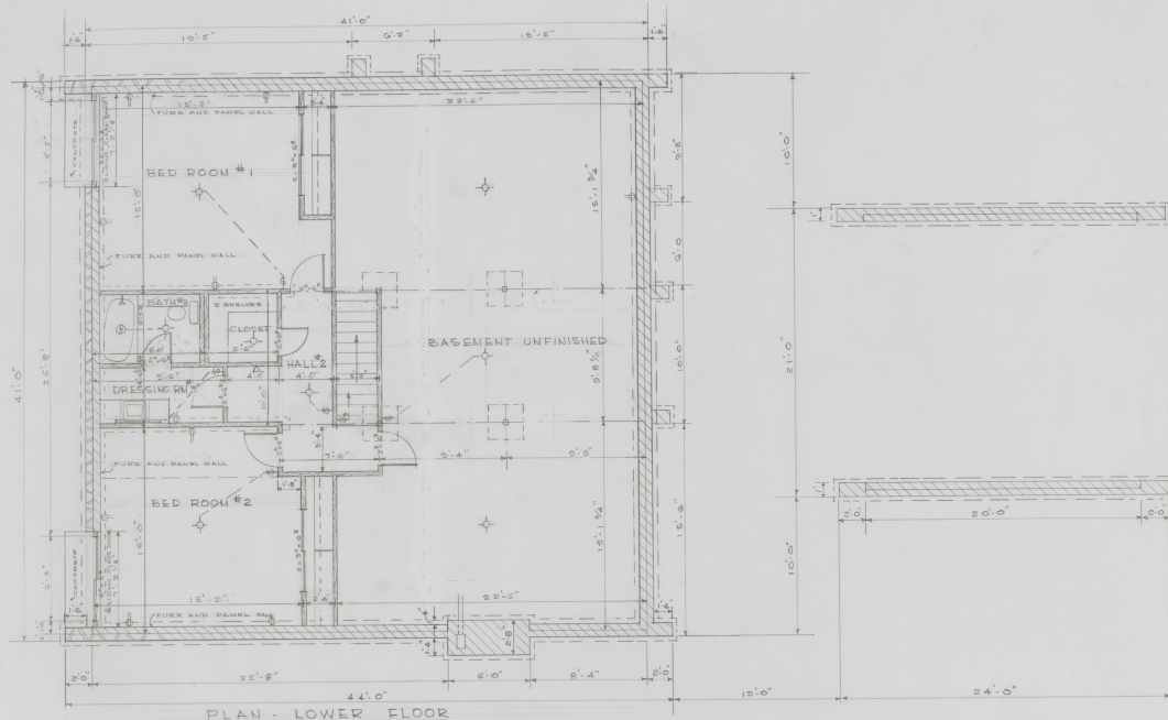
PLAN - LOWER FLOOR
