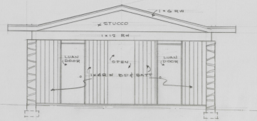
CARPORT RIGHT SIDE ELEV.
