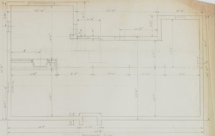
BASEMENT PLAN
