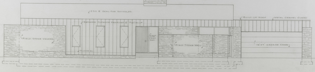
FRONT ELEVATION NOTE: GARAGE ROTATED TO SHOW ACTUAL FRONT ELEV. 1/4" = 1'-0"
