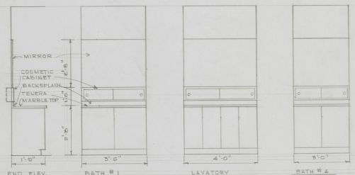
BATH VANITY ELEVATIONS 1/2" = 1'-0"
