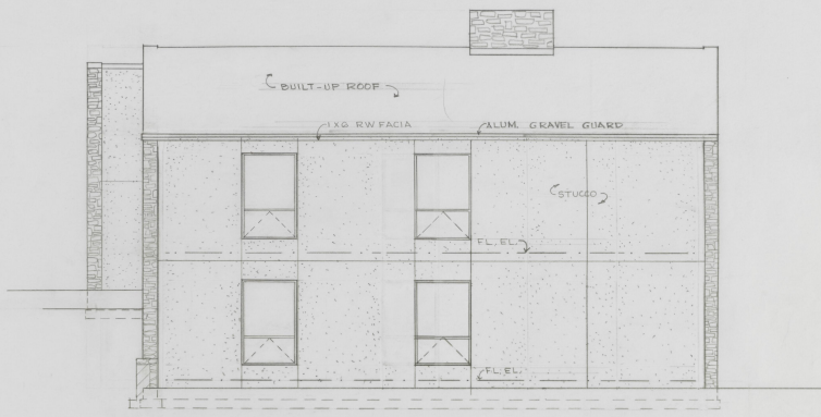
RIGHT SIDE ELEVATION 1/4" = 1'-0"
