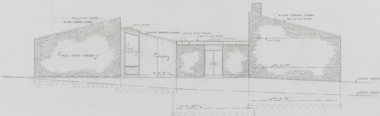
FRONT ELEVATION
