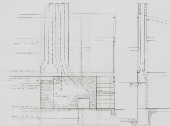
SECTION - LIVING ROOM FIREPLACE 1/4" = 1'-0"
