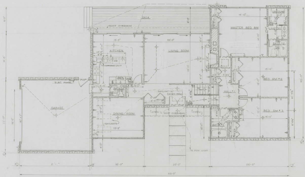
PLAN - UPPER LEVEL 1/4" = 1'-0"
