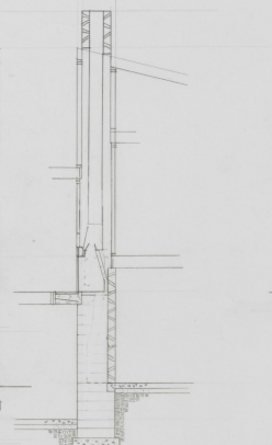
SECTION - LIVING ROOM FIREPLACE 1/4" = 1'-0"
