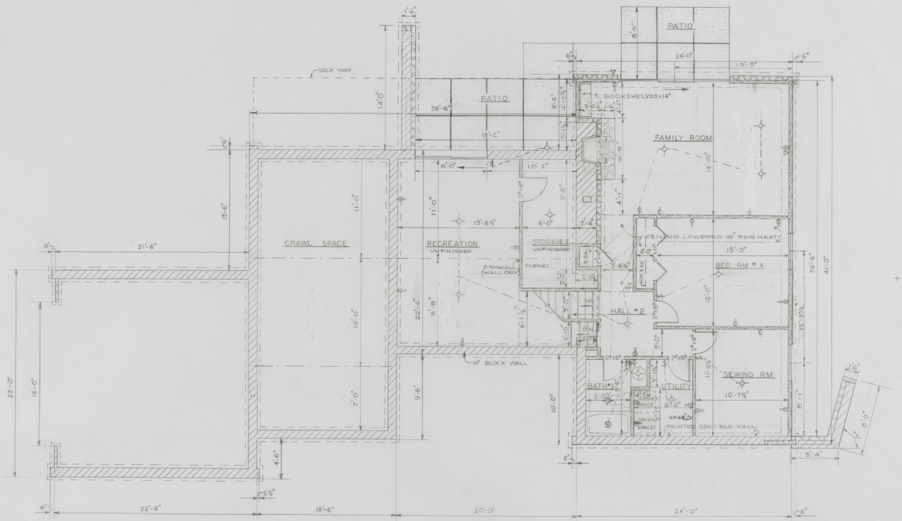
PLAN - LOWER LEVEL 1/4" = 1'-0"
