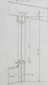
CLERESTORY SECTION 1/2" = 1'-0"
