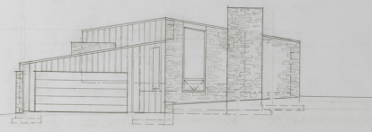
RIGHT SIDE ELEVATION 1/8" = 1'-0"
