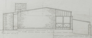
LEFT SIDE ELEVATION 1/8" = 1'-0"
