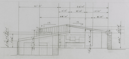
SECTION - FAMILY ROOM 1/8" = 1'-0"
