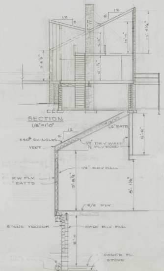
WALL SECTION 1/4" = 1'-0"
