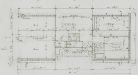
FOUNDATION PLAN
