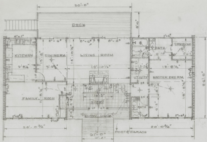
MAIN FLOOR PLAN 1/8" = 1'-0"
