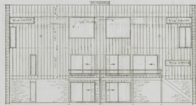
REAR ELEVATION
