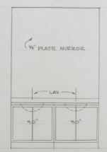
BATH #2 VANITY ELEVATION 1/2" = 1'-0"
