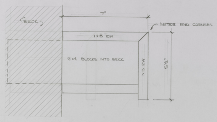
MANTEL BEAM SECTION 1/2" = 1"
