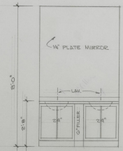
BATH #1 VANITY ELEVATION 1/2" = 1'-0"
