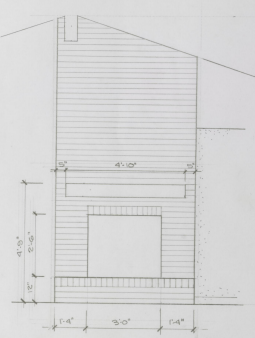
FAMILY RM FIREPLACE ELEVATION 1/4" = 1'-0"
