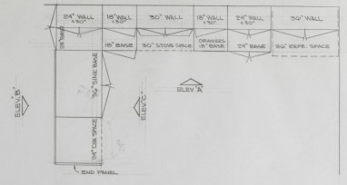
KITCHEN CABINET PLAN 1/2" = 1'-0"
