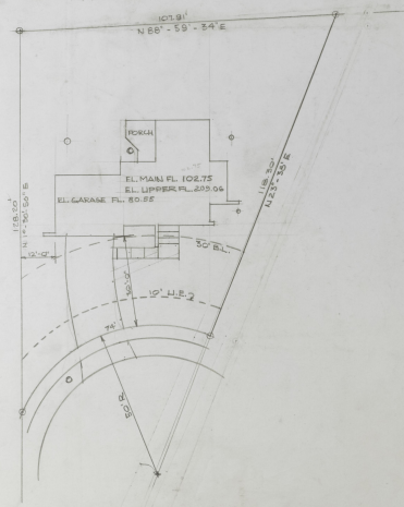
PLOT PLAN 1/4" = 1'-0"
