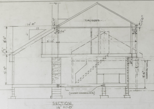
SECTION 1/4" = 1'-0"
