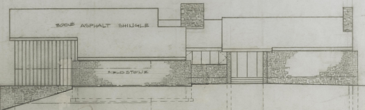
EAST ELEVATION SCALE 1/8" = 1'-0"
