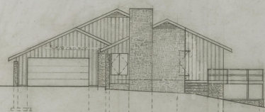
NORTH ELEVATION SCALE 1/8" = 1'-0"
