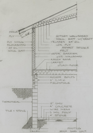
FAMILY ROOM SECTION SCALE 1/8" = 1'-0"
