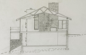
DINING ROOM SECTION SCALE 1/8" = 1'-0"
