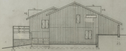
SOUTH ELEVATION SCALE 1/8" = 1'-0"
