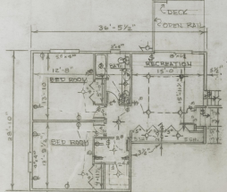
LOWER LEVEL SCALE 1/8" = 1'-0"
