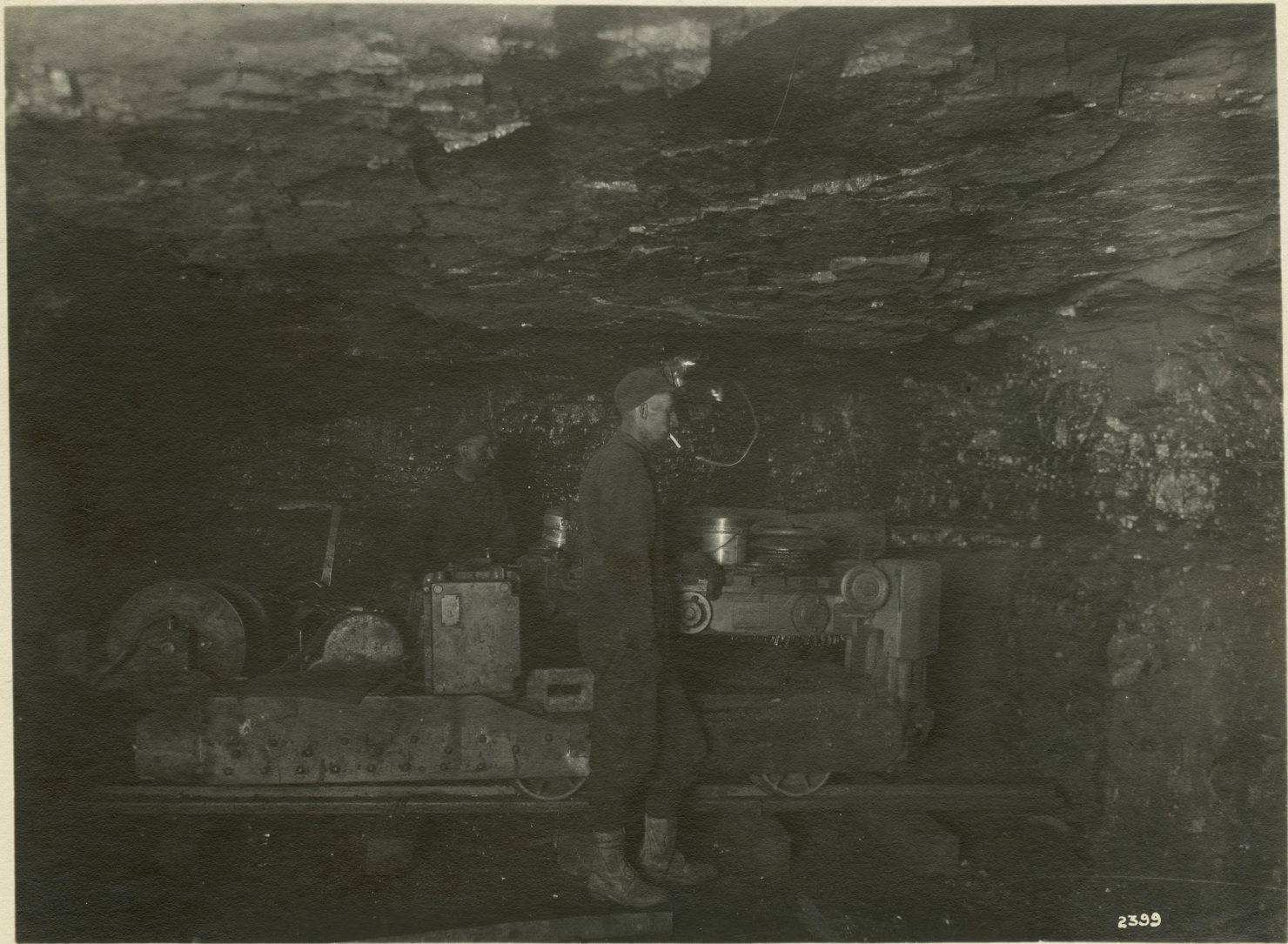
Arc-wall Mining Machine in Operation, 8-4-23.
