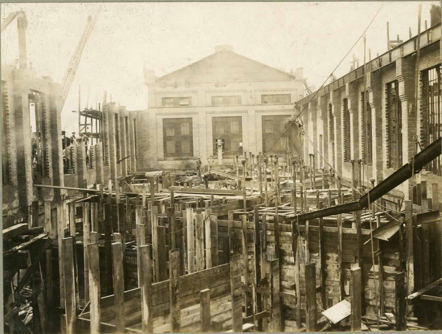
Completed Engine Foundation ~ Dec. 23, 1914
