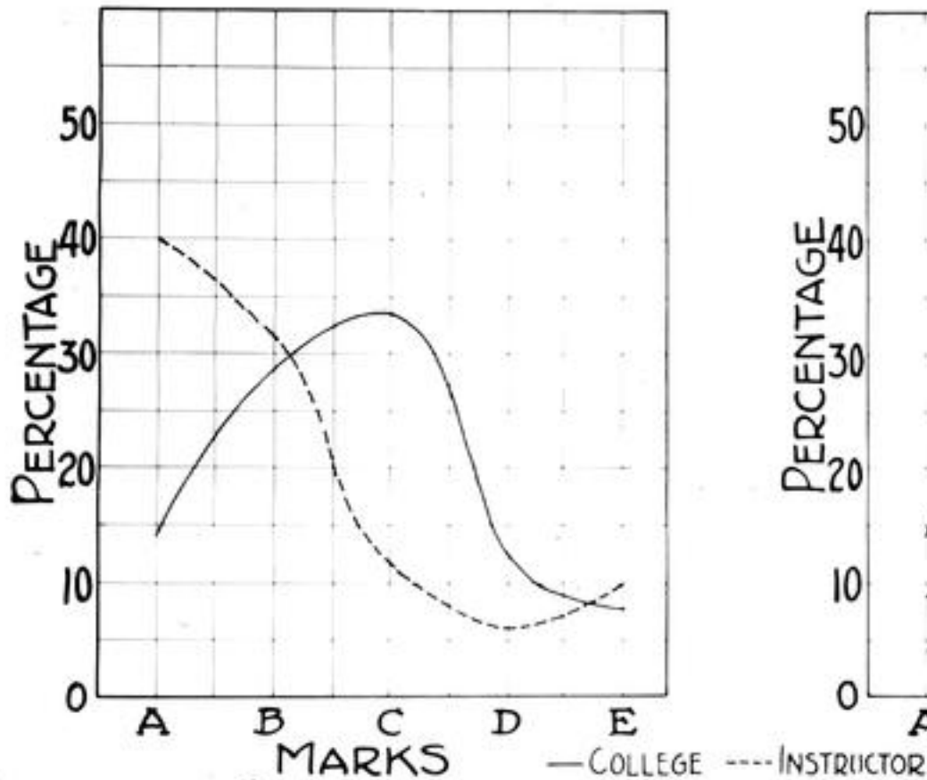
COMPARISON OF THE PERCENTAGE DISTRIBUTION OF MARKS OF AN INSTRUCTOR WHO GIVES FEW HIGH AND FEW LOW MARKS, AND THE DISTRIBUTION FOR THE COLLEGE OF ARTS & SCIENCES, 1924-25.
