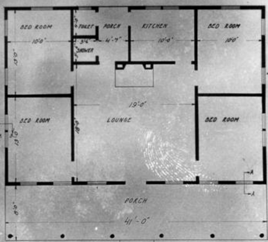
CELOTEX LODGE WILDWOOD - BY- THE - LAKE MERCER CO., KENTUCKY M. CRUTCHER - L. H. McCAN - C. D. DICKERSON - D. Y. TERRELL. Hugh Meriwether, C. E. - Architect. Louisville - - - Lexington.
