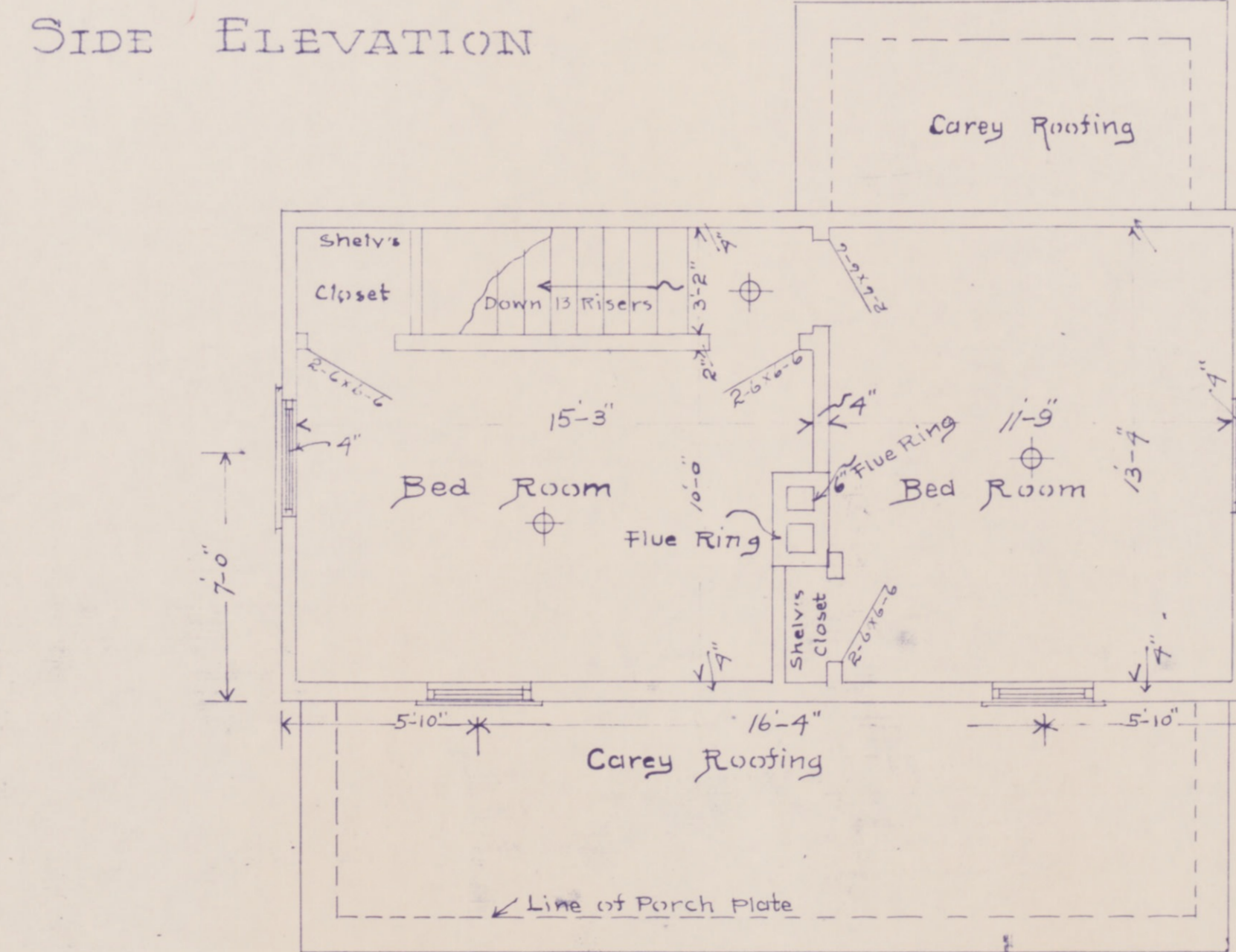
SECOND FLOOR PLAN SCALE 1/4 INCH ONE FOOT
