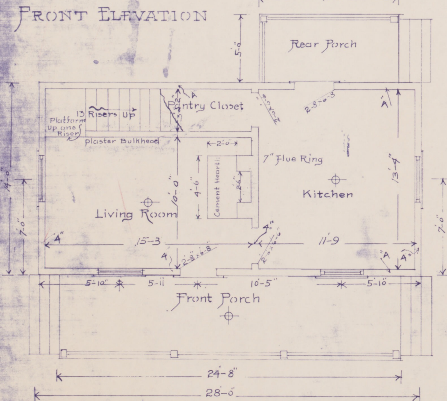
FIRST FLOOR PLAN SCALE 1/4 INCH ONE FOOT
