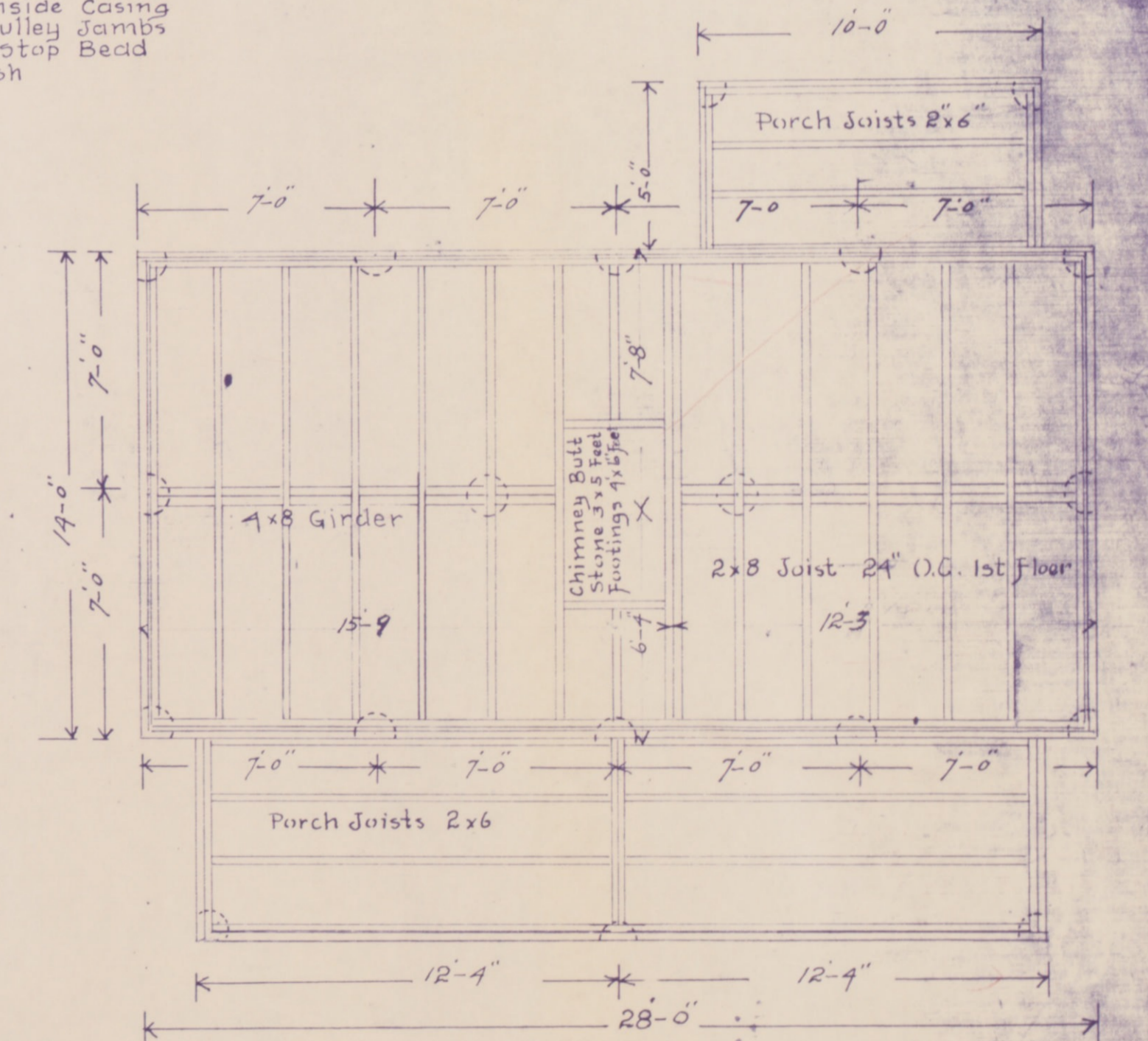
FOUNDATION PLAN SCALE 1/4 INCH ONE FOOT
