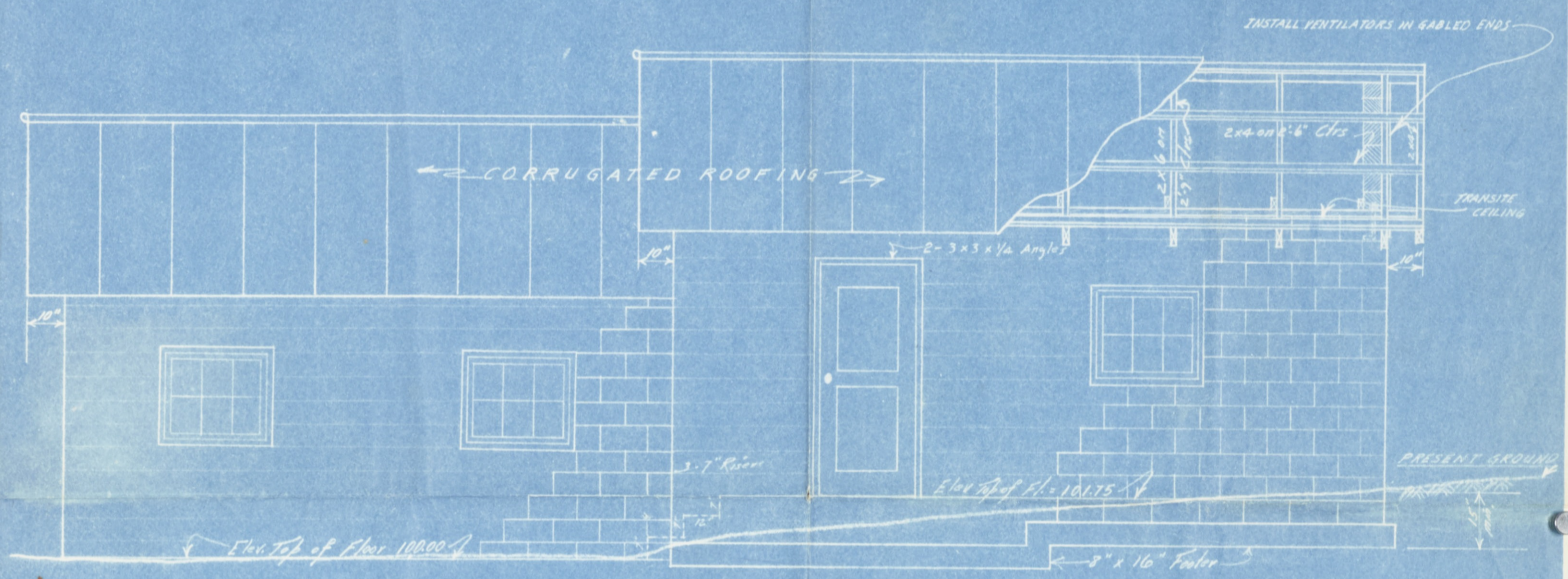
SOUTH ELEVATION
