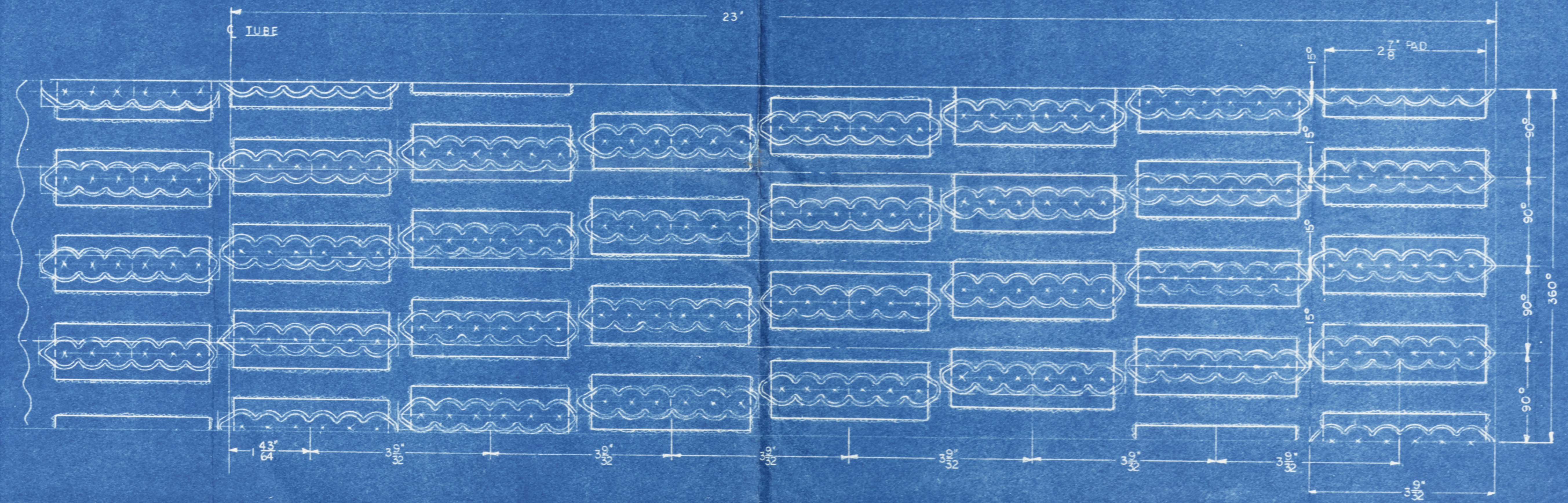
DEVELOPMENT OF ONE HALF BRUSH MOUNTING BRUSH ROTATES 210° IN 48°
