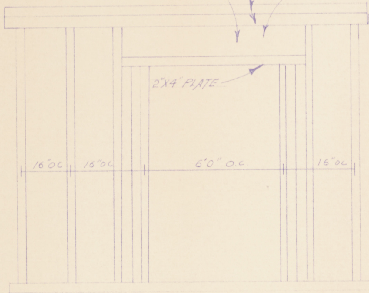
FRAMING DETAIL ENTRANCE OFFSET (NOT TO SCALE)
