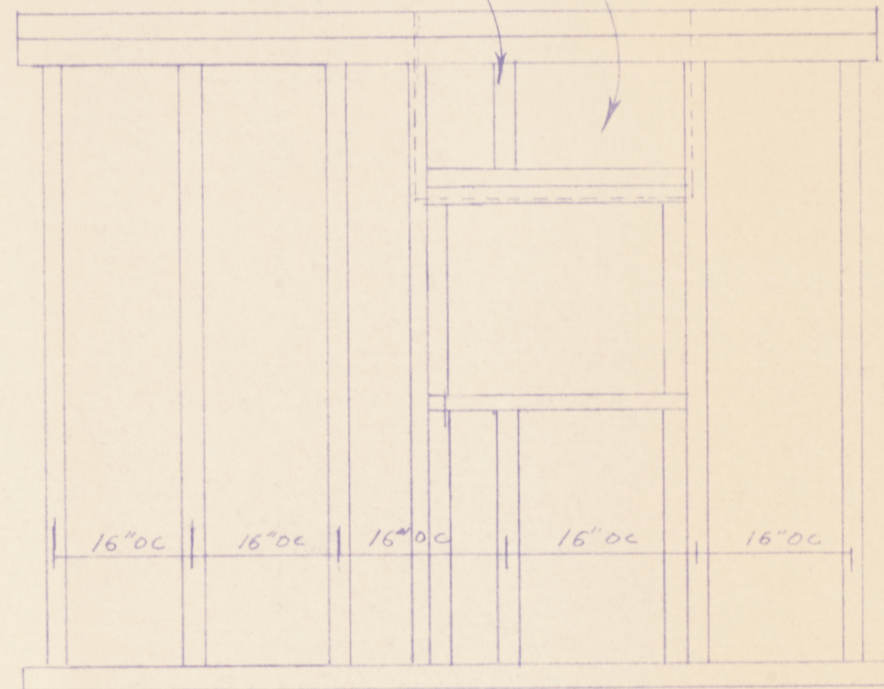
WINDOW FRAMING DETAILS (NOT TO SCALE)
