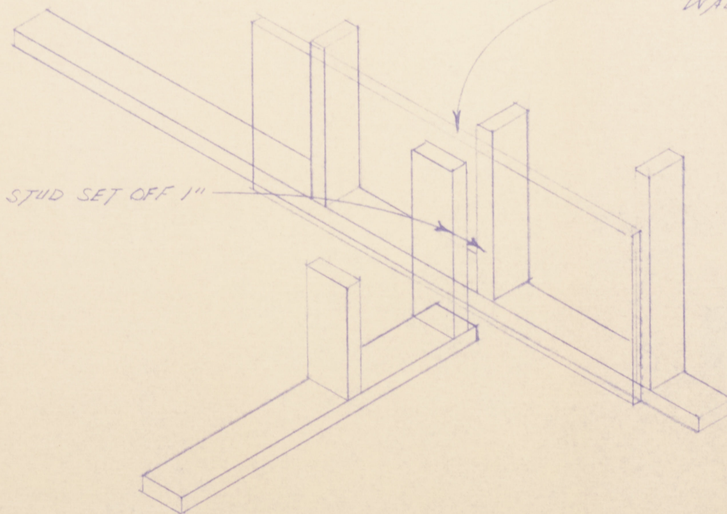
INTERIOR WALL FRAMING DETAIL (NOT TO SCALE)
