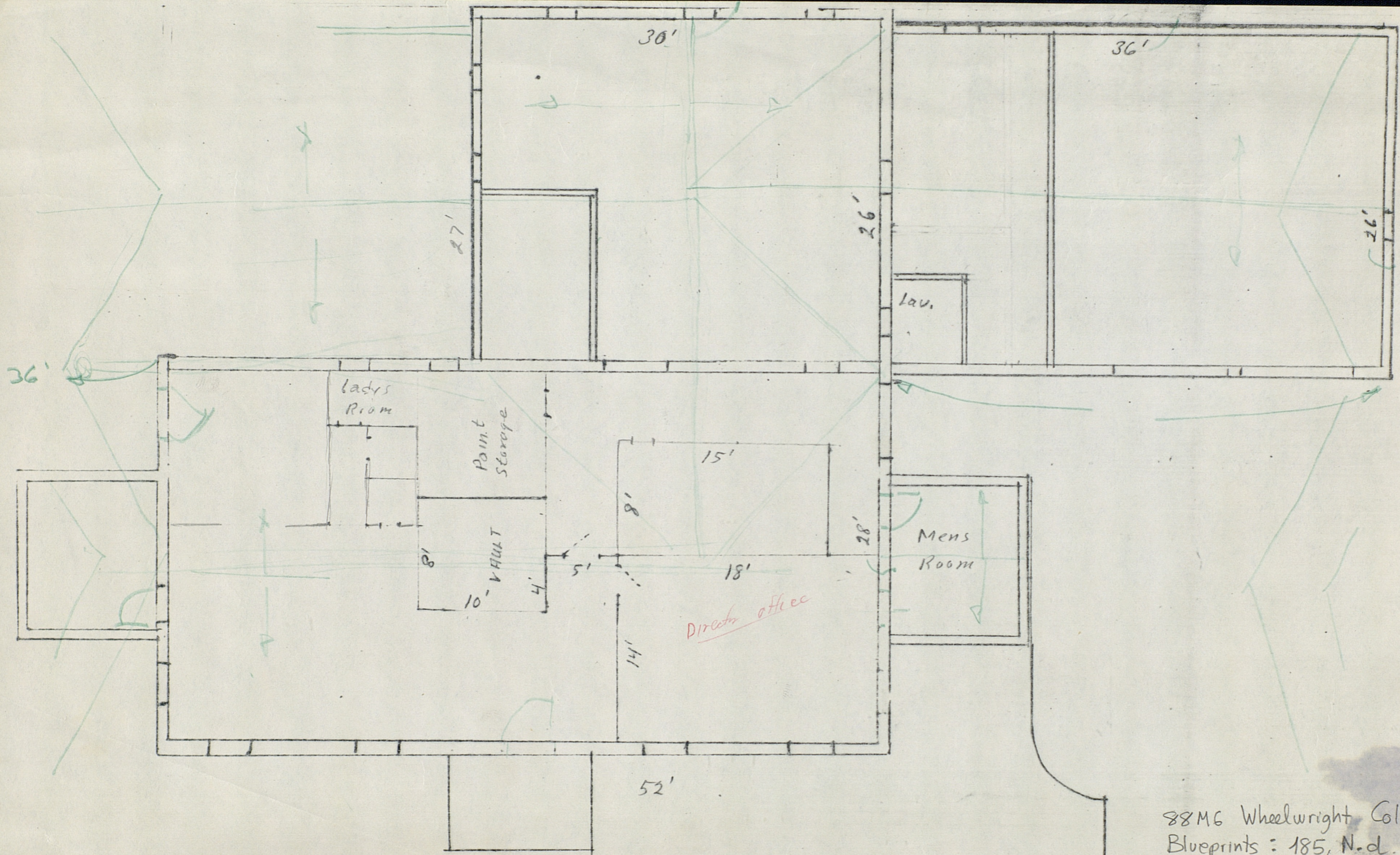
FLOOR PLAN - CENTRAL OFFICE / MAINTENANCE - R11
