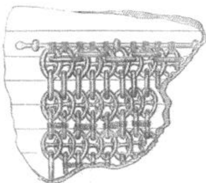
SECTION OF CHAIN ARMOR PLACED ON THE SIDE OF THE "BROOKLYN" TO PROTECT HER BOILERS. FROM A SKETCH LENT BY COMMANDER BARTLETT.
