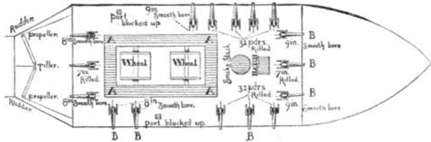
THE PLAN OF THE "LOUISIANA." AFTER A SKETCH MADE BY COMMANDER J. K. MITCHELL ABOUT THE TIME OF THE ENGAGEMENT.
